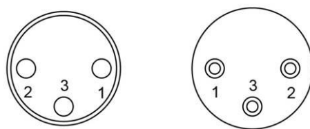
3 Pin XLR
